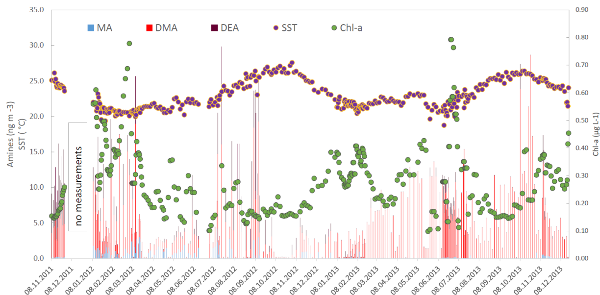
Figure 1: Time series of the particulate amine concentrations, in detail: MA – monomethyl amine, DMA - diethyl amine and DEA - diethyl amine (ng m -3 ) together with chl-a (µg L -1 ) and the SST (°C) for the 24-month time series measured at the CVAO.
